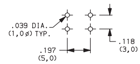
PC MOUNTING
