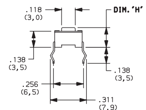
PTS635SL43 SPST
