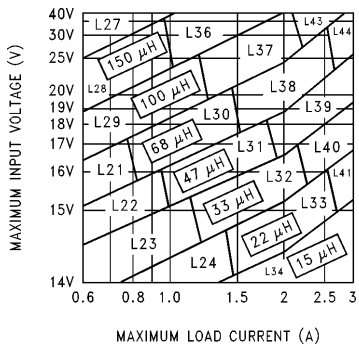
FIGURE 7. LM2596-12
